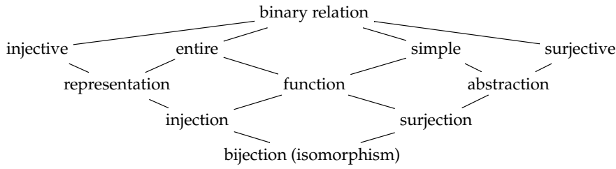
Figure 5.1.: Binary relation taxonomy
