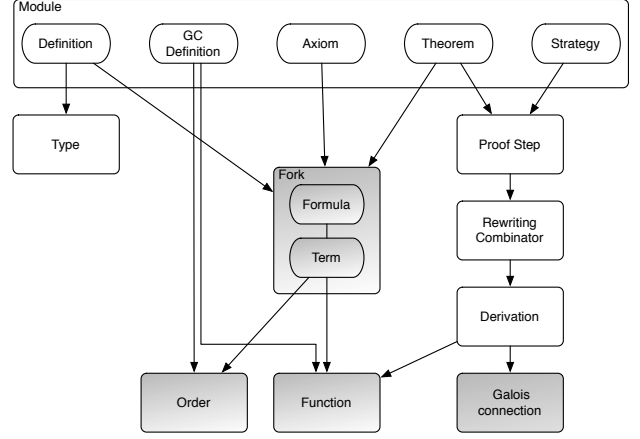
Figure 1. Structure of the sub-languages of the Galois DSLs. The arrows represent inclusion between languages; the shaded boxes are the fragments described in this paper.
