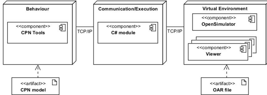
Fig. 1. Logical architecture of the APEX framework
