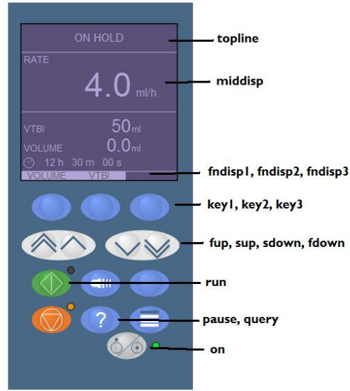
Fig. 3 Alaris actions(see [33])
